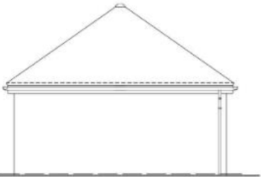
Proposed Side Elevation Scale 1:50
