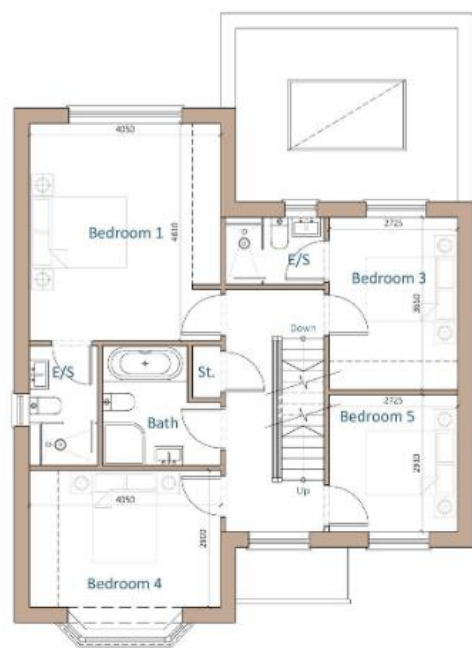
Proposed First Floor Plan Scale 1:50
