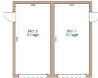
Proposed Ground Floor Plan Scale 1:50
